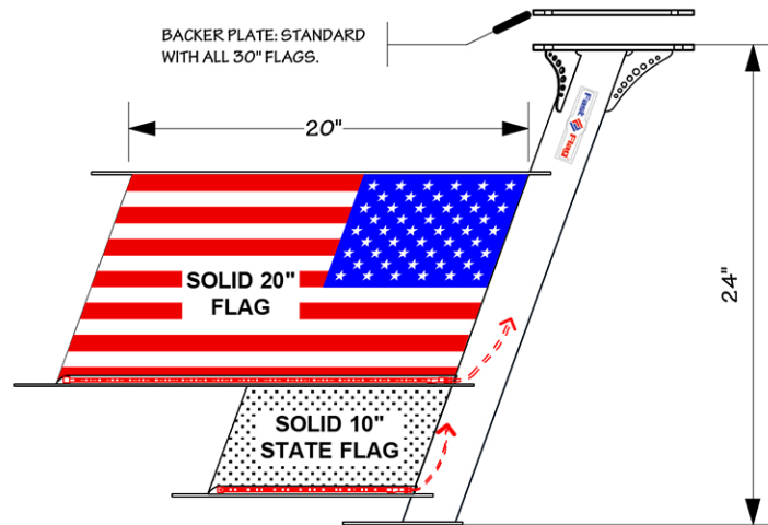
STARBOARD SIDE VIEW
