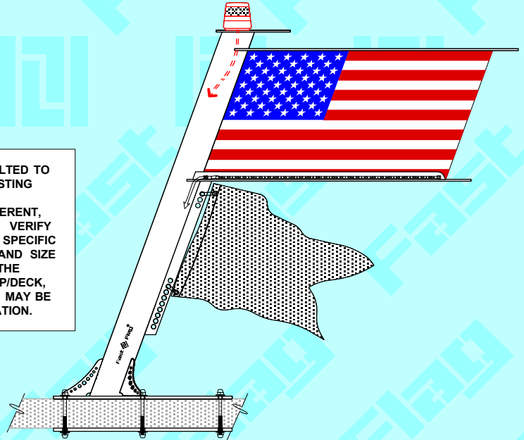
SSB-20 FIXED BASE SOLID
