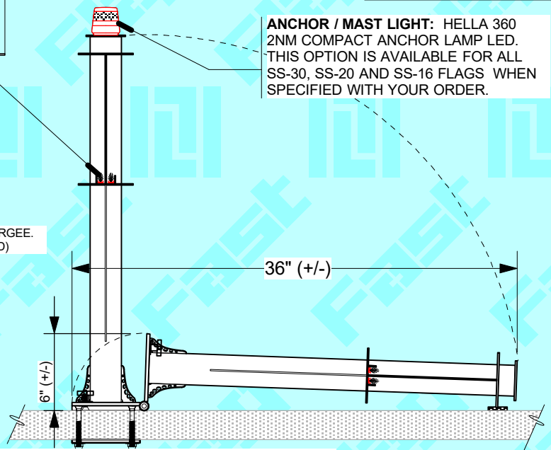
SSB-20FDB SOLID/STENCIL (AFT VIEW)
