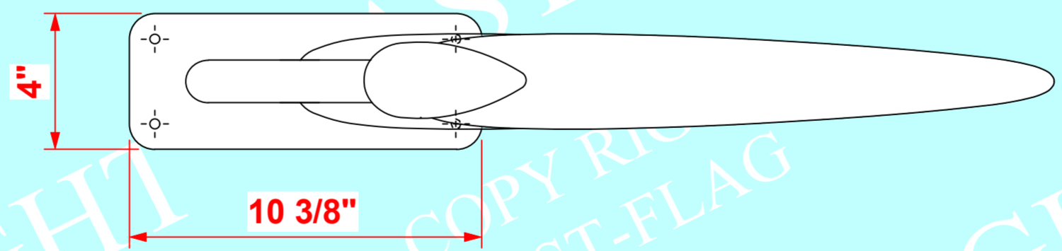
TOP VIEW
